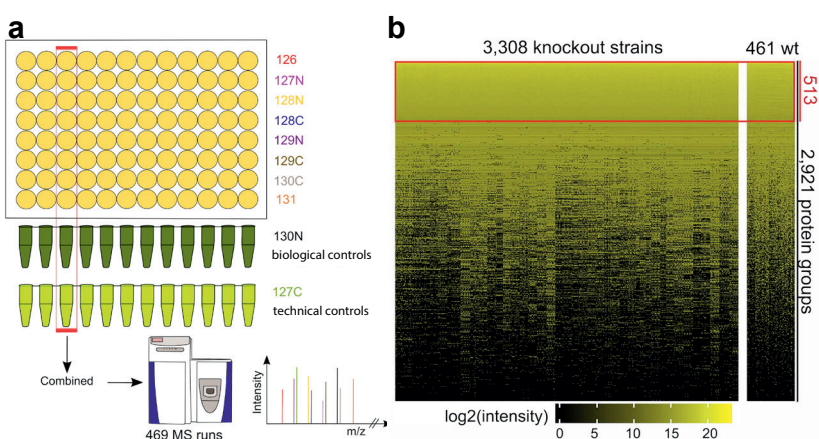
Figure 1. Studying the proteome across a complete knockout library. A) Schematics of the experimental design for quantifying protein expression levels in the S. pombe knockout collection by quantitative proteomics using 10plex tandem mass tags. B) Normalised protein expression levels of 3,308 knockout strains and 461 wild-type replicates. The complete dataset contains the quantification of 2,921 protein-coding genes, of which 513 proteins were quantified across all samples. (Öztürk et al , 2022, Nat Commun ).
