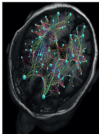
Structural Connectome from T1 and diffusion MRI
