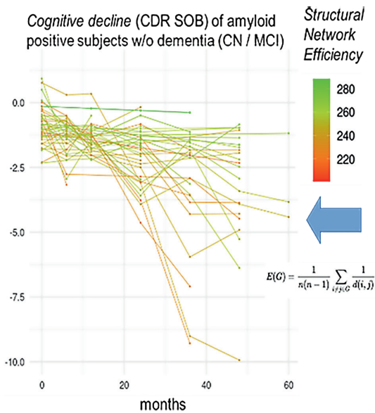
Structural Connectome from T1 and diffusion MRI
