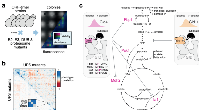
Figure 1. Systematic characterisation of the ubiquitin-proteasome system. A) Proteomic profiling of the yeast UPS in colony arrays expressing different fluorescent timer-tagged proteins and carrying mutations in individual UPS components. B) Correlations between the proteome turnover profiles of UPS mutants highlight functional relationships between UPS components. C) Model of bidirectional control of the switch between glycolysis and gluconeogenesis by GID complexes.
